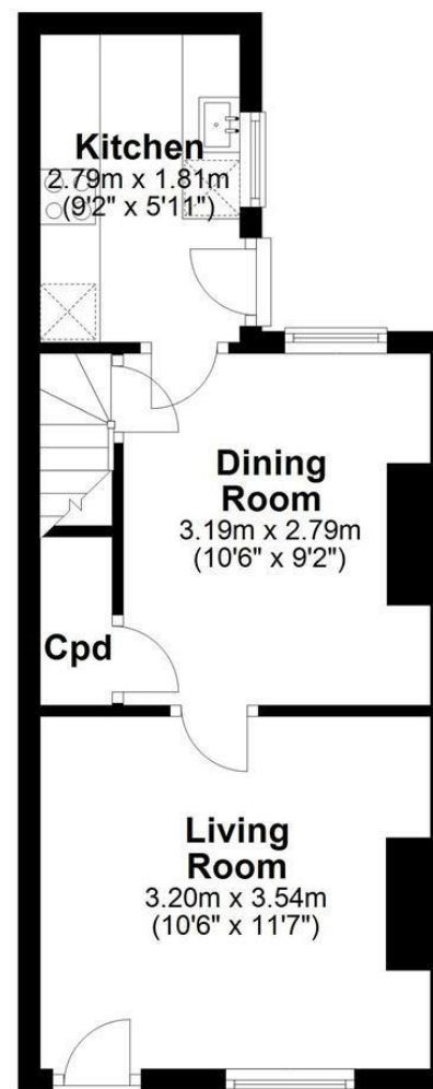
Ground Floor Approx. 28.2 sq. metres (303.8 sq. feet)
